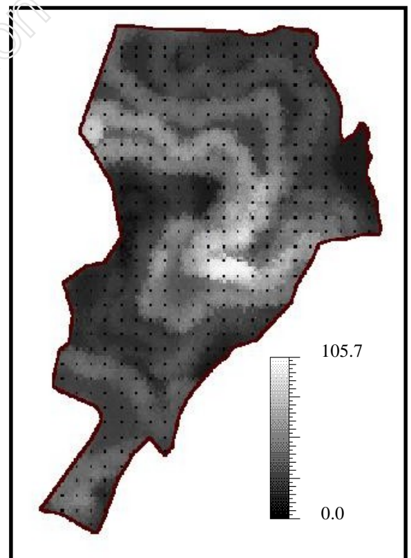
Figure 9: Map of local uncertainties based on interdecile confidence intervals ( \text{Prob}\{Z(u) \in [q_{0.10};q_{0.90}]\} = 0.8 )
