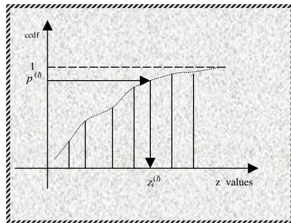
Figure 2: Process of obtaining a realization from a estimated univariate ccdf
