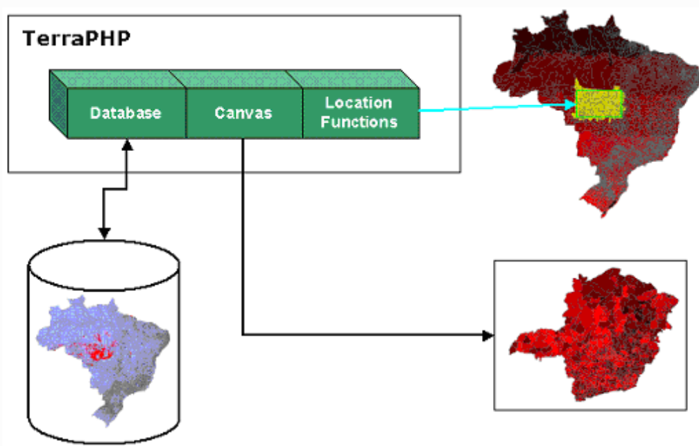
Figure 1 - TerraPHP Architecture
