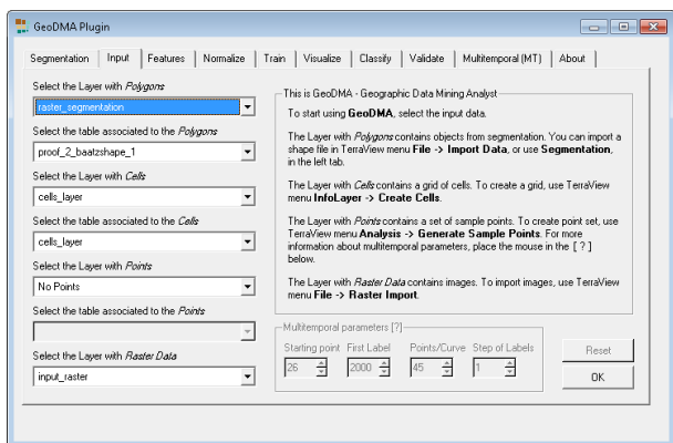
Figure 1: User interface for GeoDMA.
