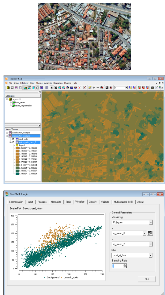
Figure 8: The input image (top), visualization tools using a map of features (middle), and a scatterplot (bottom). The map shows the feature ratio of band 1, showing it is a proper feature to distinguish the target Trees. The scatterplot shows the feature space of features mean of bands 0 and 2, distinguishing the target Roofs from the rest of the image.
