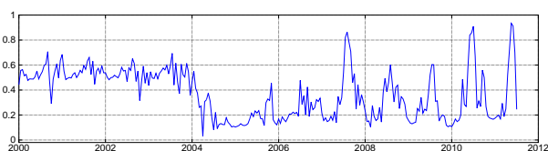
Figure 3: EVI2 profile example from 2000 to 2011, the range of values is [0,1]. Adapted from [25].
