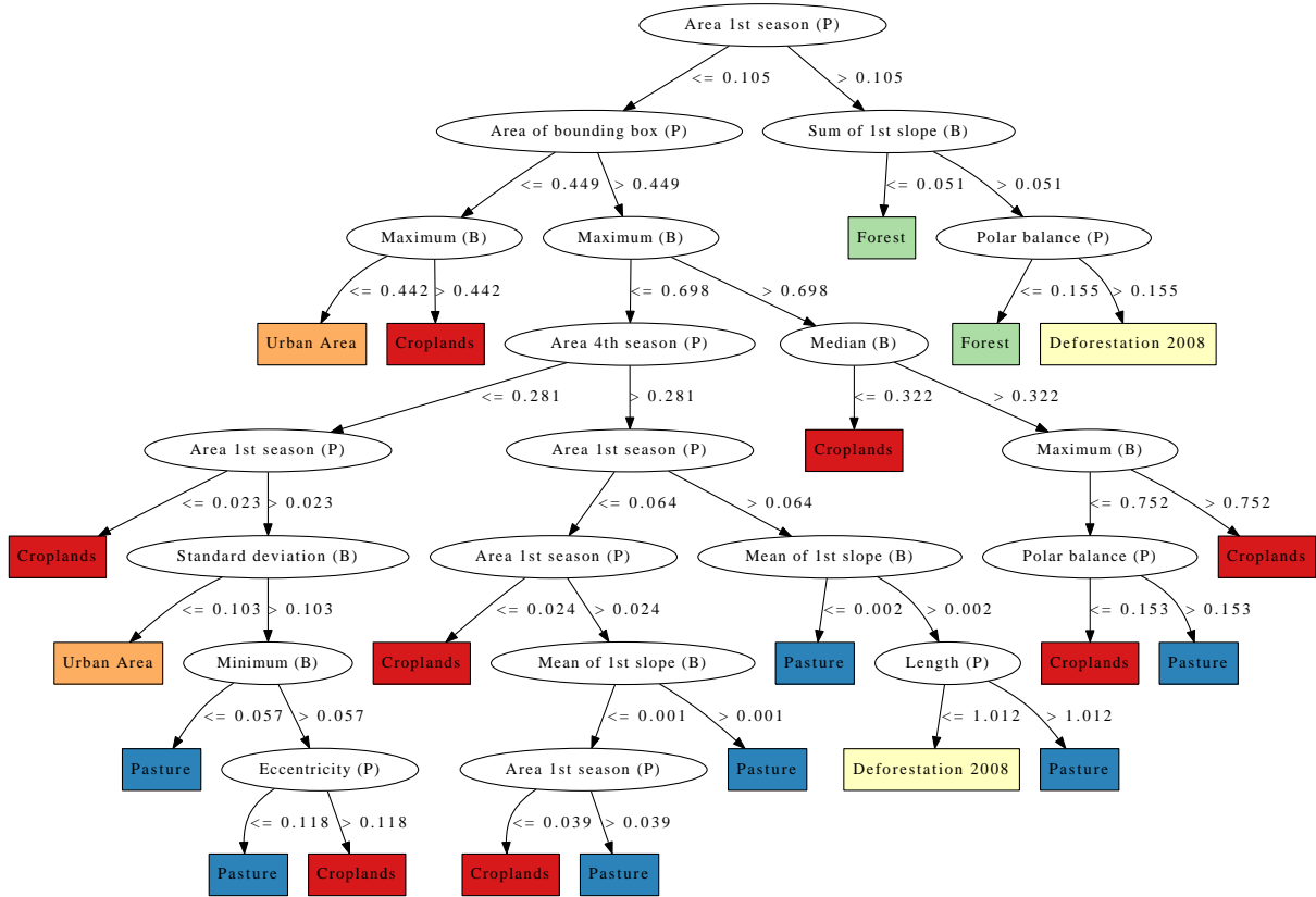
Figure 12: Classification model for the second experiment, with 13 leaves and Kappa = 0.82.
