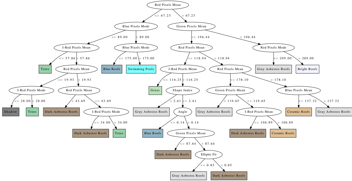
Figure 10: The decision tree model for intra-urban land cover classification in a region of São Paulo city, Brazil.
