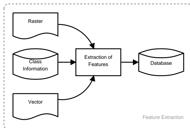
Figure 4: Feature extraction – Spectral and Spatial features use raster and vector information. Landscape ecology features use class information. Multi-temporal features use cycles’ information.
