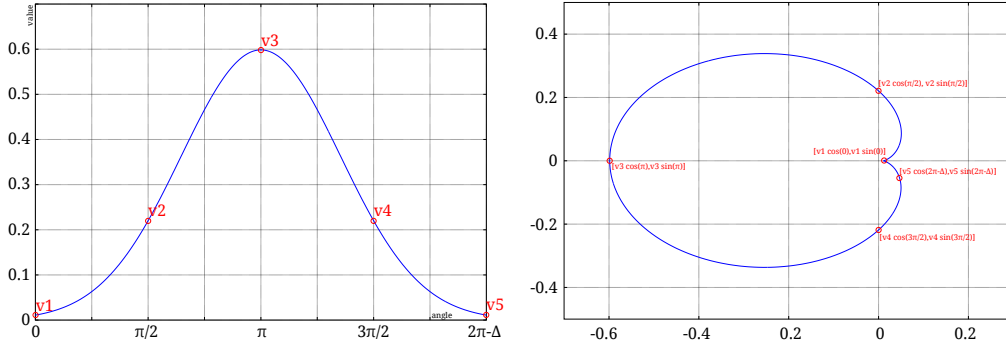
Figure 6: When the values of the cycle are associated to a certain angle (left), the closed shape is created from its polar transformation (right).
