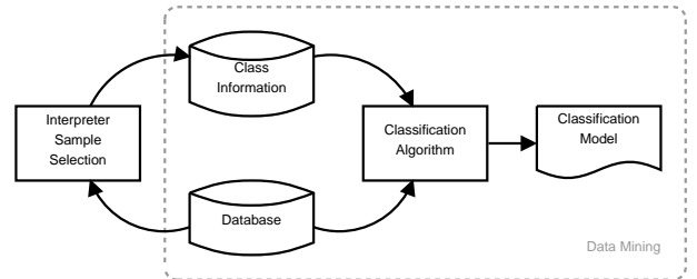
Figure 7: The interpreter defines a typology and the set of representative samples, which are used to create the classification by applying the data mining algorithm.
