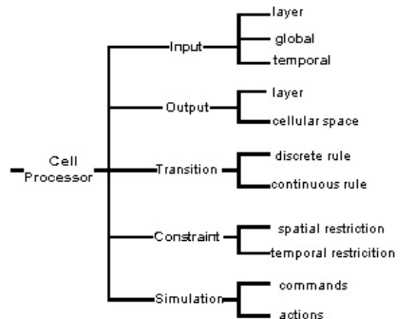
Figure 4 the TerraML Simplified Structure
