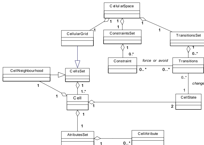
Figure 7 The cellular space class hierarchy
