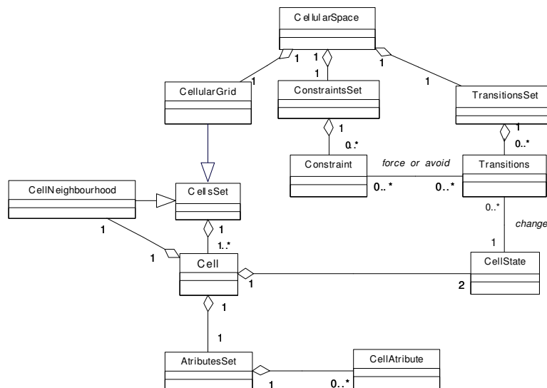
Figura 7 The cellular space class hierarchy
