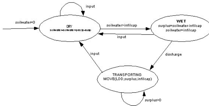
Figure 1 A water balance hybrid automaton
