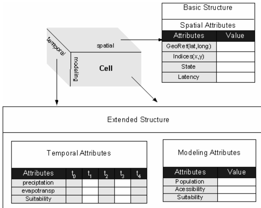
Figure 3 The Cell-Space Data Structure in TerraML
