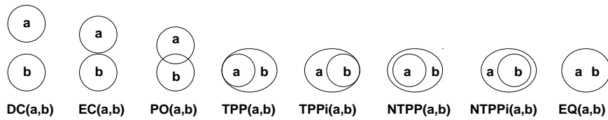
Figure 3. Illustrations of eight JEPD relations
