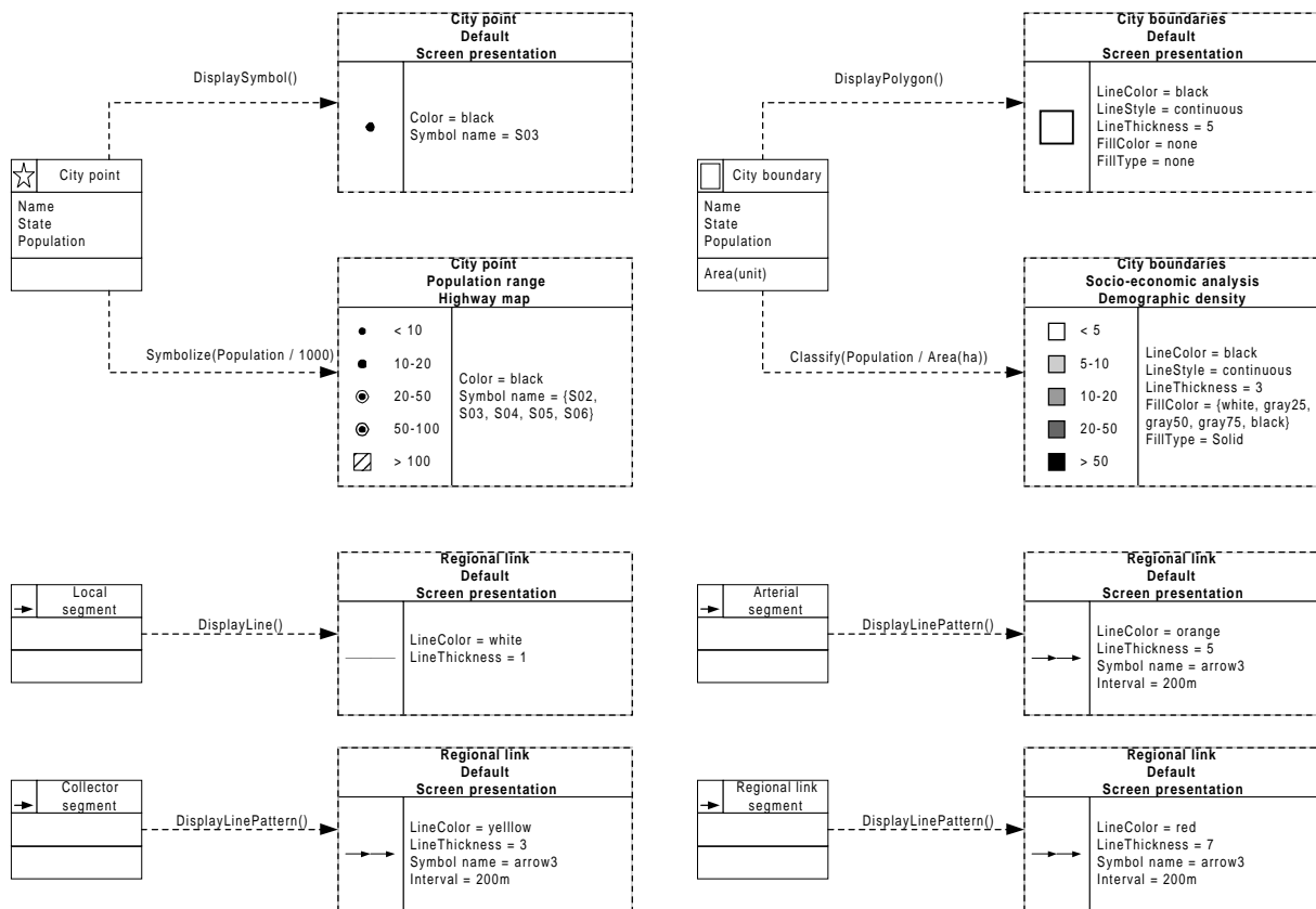
Figure 23 - Presentation diagram fragment for the example
