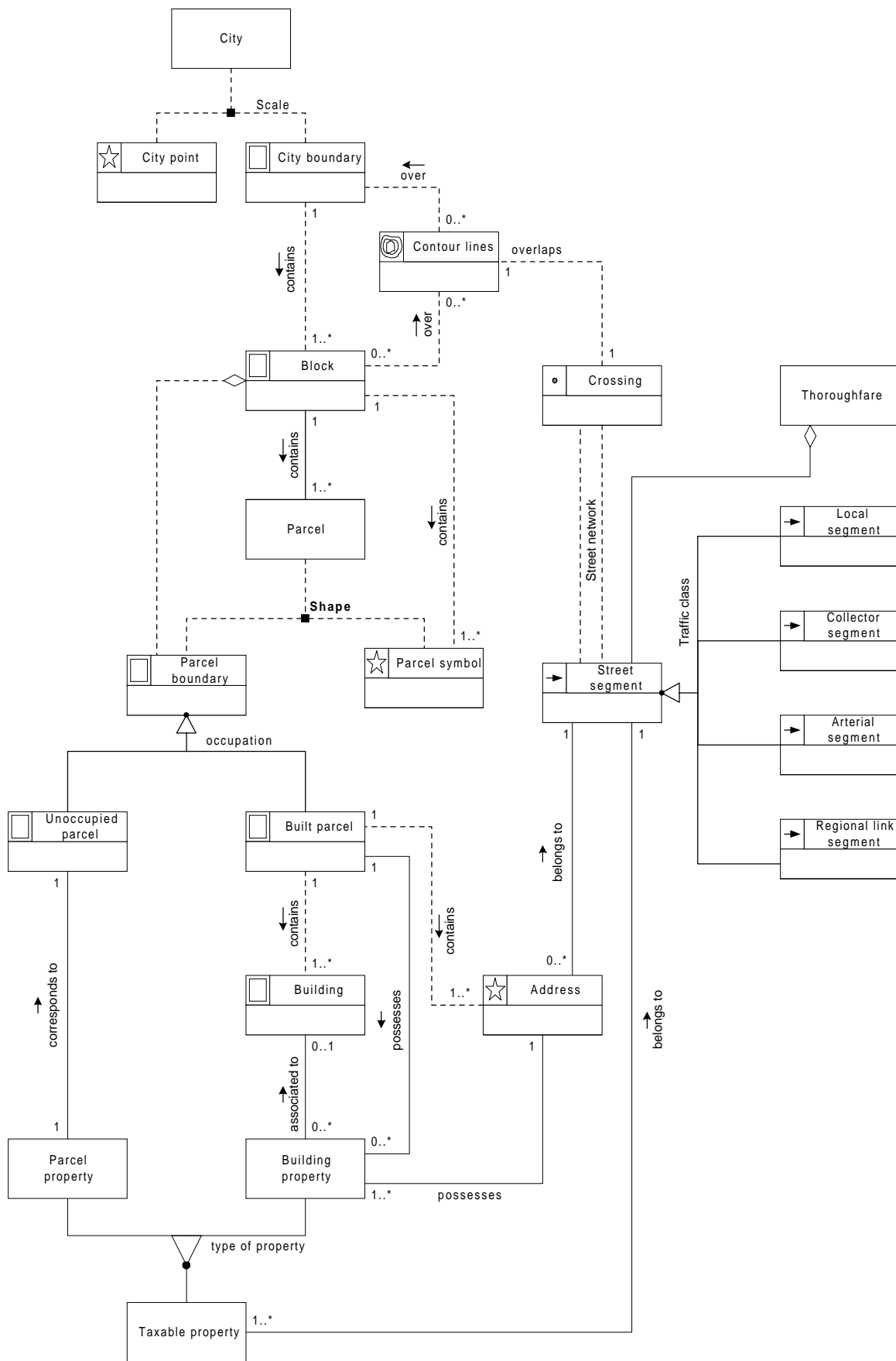
Figure 21 - Partial class diagram of the urban cadastral database
