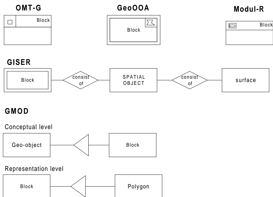
Figure 25 - Geo-object schema (polygon - block)
