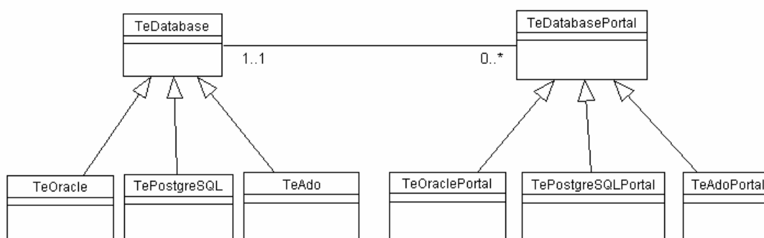
Figura 3.2 - Interface com SGBDs
